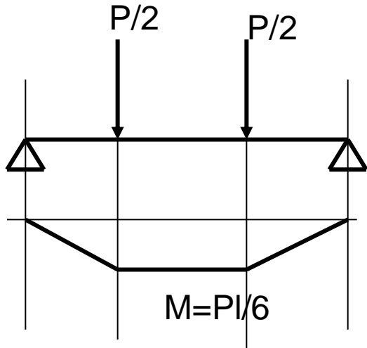
FIGURE 7.13 Apparatus for flexure test of concrete by third-point loading method. Copyright ASTM. Reprinted with permission.
