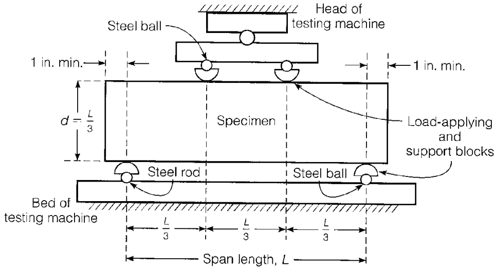
FIGURE 7.13 Apparatus for flexure test of concrete by third-point loading method. Copyright ASTM. Reprinted with permission.
