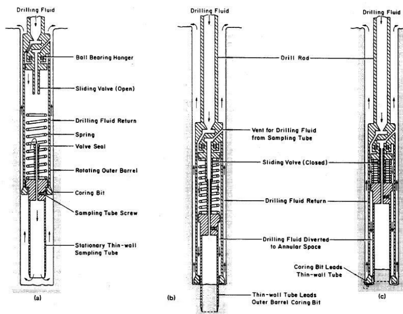
Pitcher Sampler: (a) Sampler Being Lowered into Drill Hole; (b) Sampler During Sampling of Soft Soils. (c) Sampler During Sampling of Stiff or Dense Soils. (Courtesy of Mobile Drilling, Inc.)
