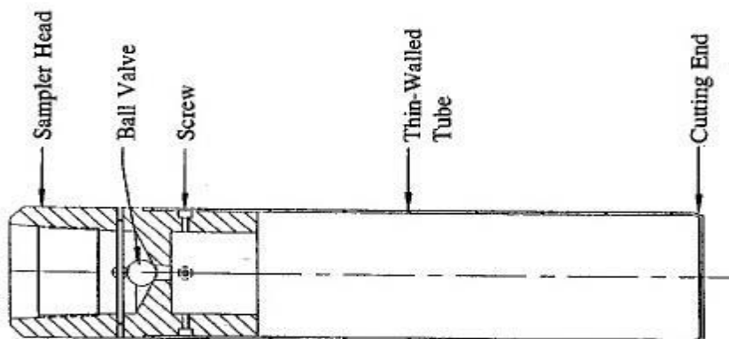
Schematic of Thin-Walled Shelby Tube (After ASTM D 4700).
